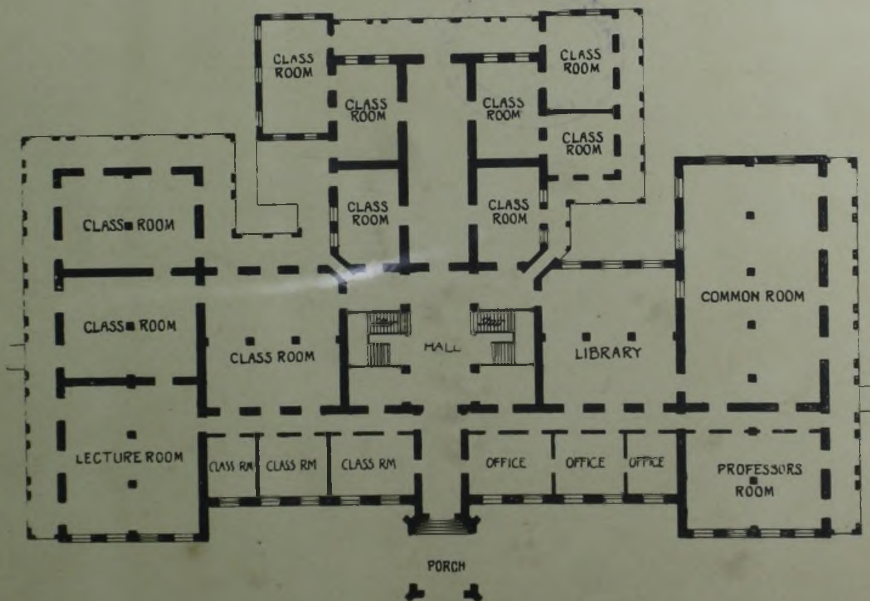
GROUND PLAN
