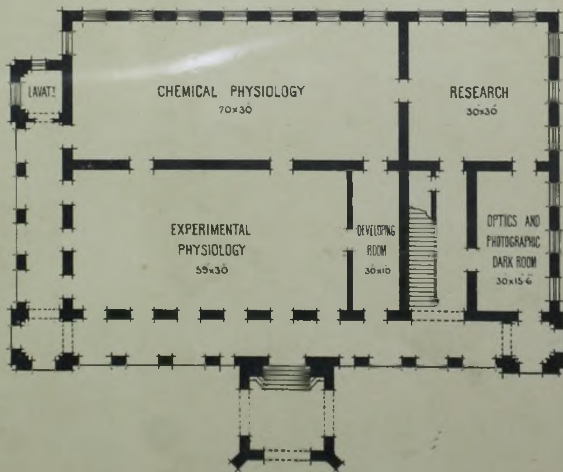
GROUND PLAN
