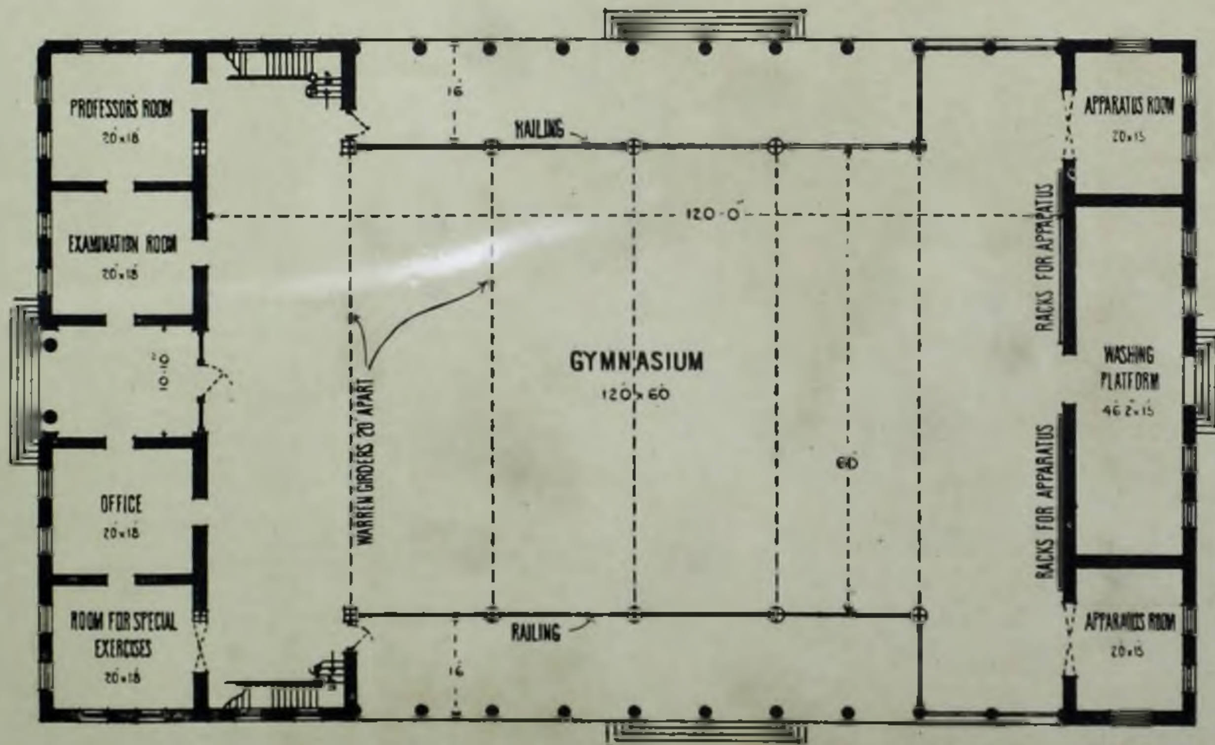
GROUND PLAN
