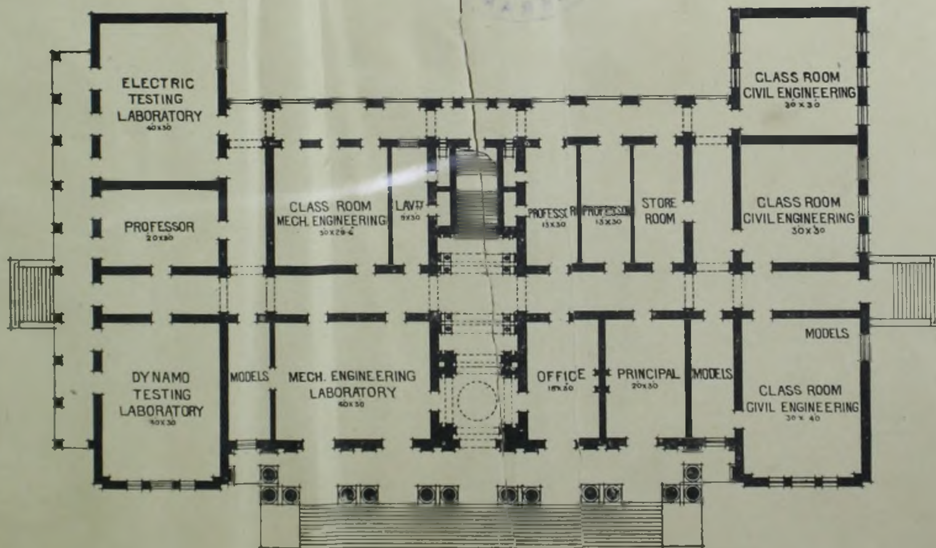
GROUND PLAN
