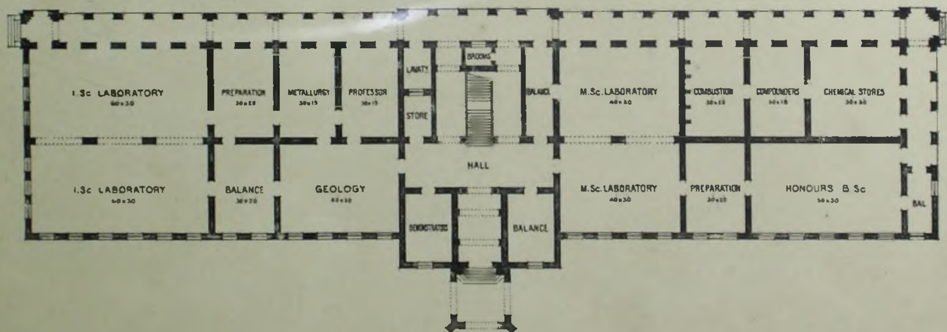
GROUND FLOOR
