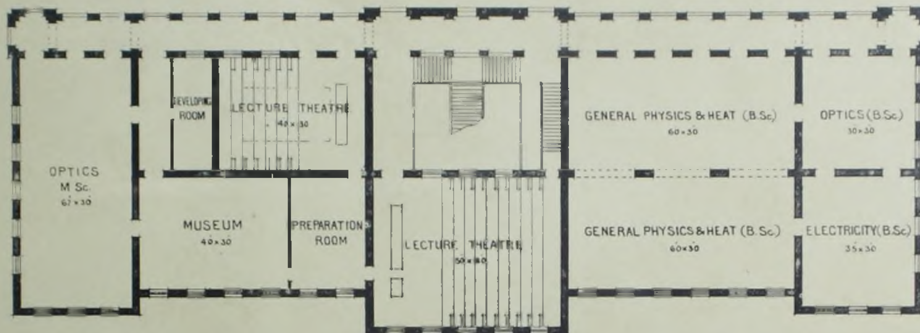
FIRST FLOOR
