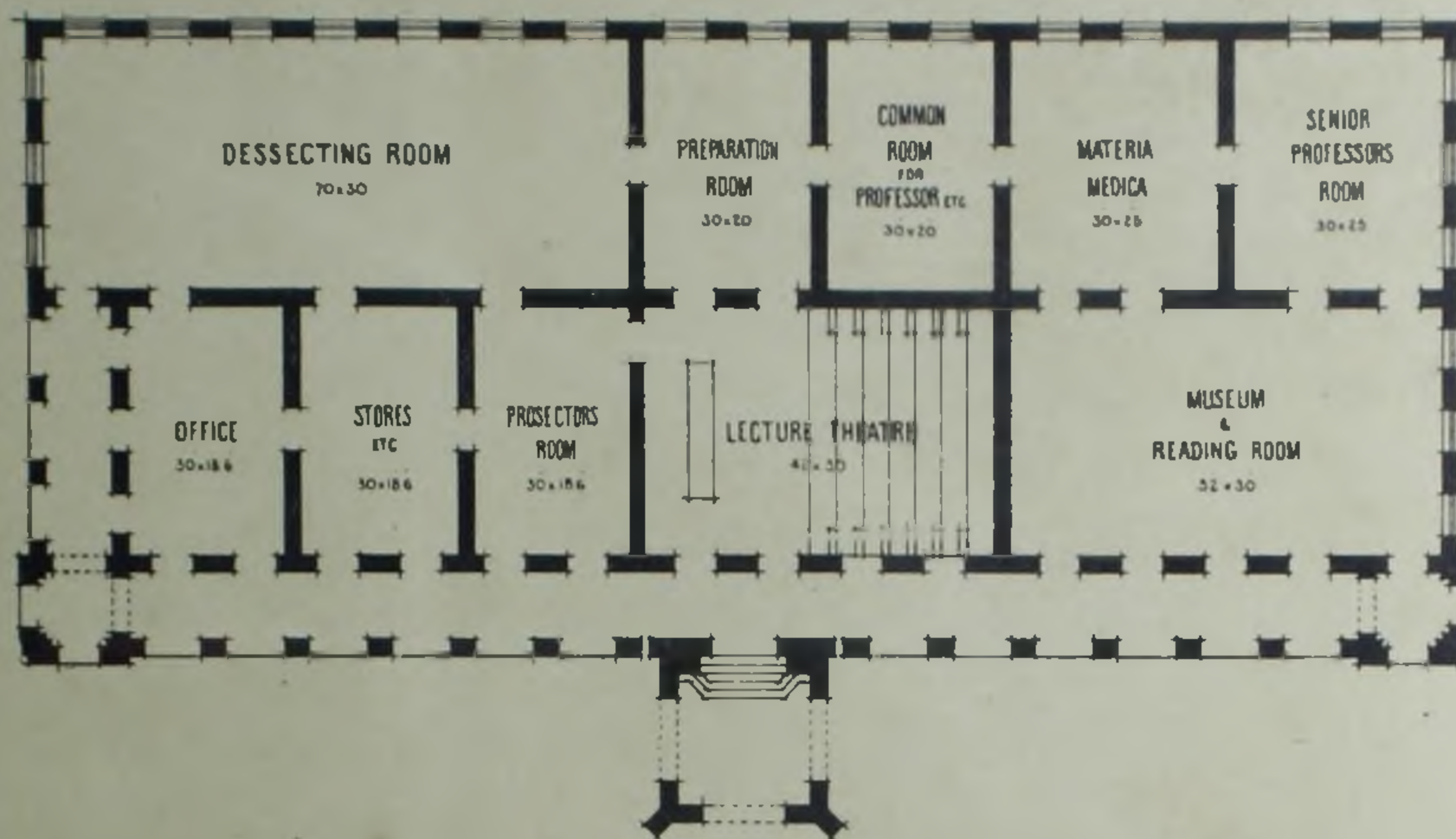
GROUND PLAN
